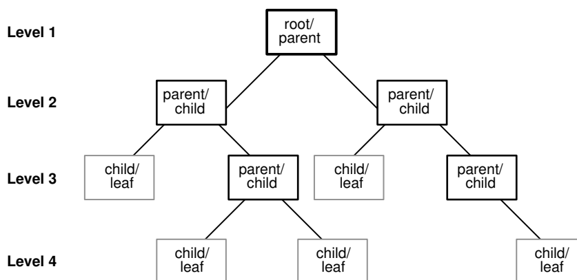
Figure 3-1 Hierarchical Tree
